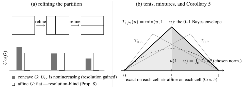
Figure 3. Saturation along the resolution axis. (a) Refining the partition can only lower the uncertainty functional U_G(G) = \mathbb{E}[G(\eta_G)] when G is concave (conditional Jensen; Blackwell [8]); the drop is the resolution term of the score decompositions [39, 10, 18]. By Proposition 8, the only uncertainty functions whose profile is flat—resolution-blind at every two-cell comparison—are the affine ones, with no regularity assumed. (b) The tent T_{1/2}(u) = \min(u, 1-u) is the 0–1 Bayes envelope; the tents T_\theta are the uncertainty functions of the elementary scores [44, 19], and the usual binary proper-score representation writes suitably normalized uncertainty functions as mixtures \int_0^1 T_\theta d\nu(\theta) ; the dashed curve is the Brier entropy u(1-u) , the uniform mixture under the chosen tent normalization. Exactness on each cell of the benchmark partition \{[0, \frac{1}{2}], [\frac{1}{2}, 1]\} forces affineness on each cell (Corollary 5): a piecewise-affine tent shape, with the familiar symmetric tent selected by endpoint and scale normalizations, pinned with nothing assumed at the kink.
